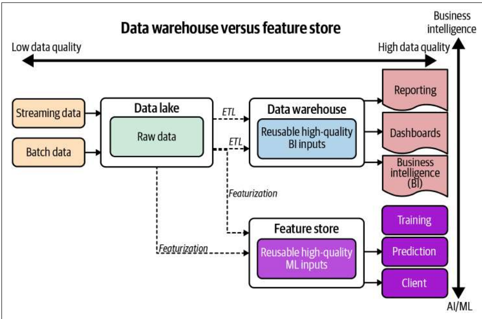
Figure 5-10. Data warehouse versus feature store
