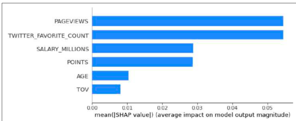
Figure 5-44. SHAP feature importance
